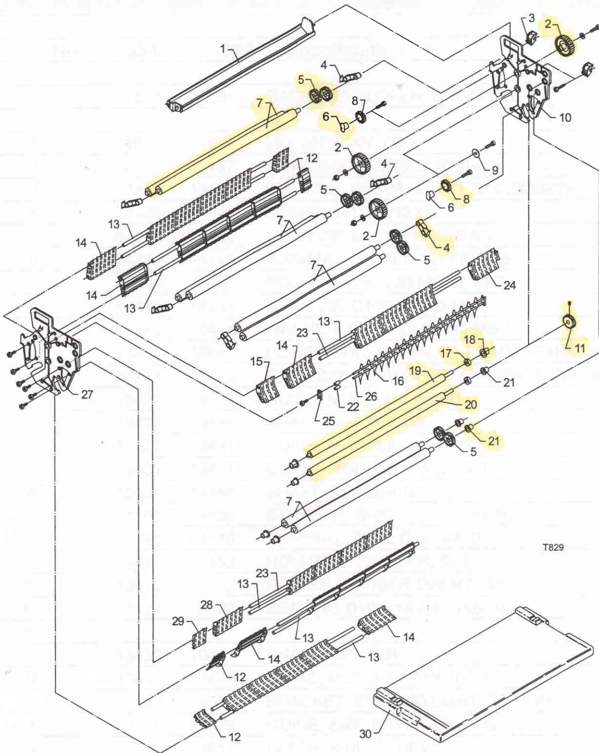
DEVELOPER RACK
